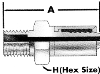
Tube Connector with Nut & Ferrule Specifications Style 31FN
