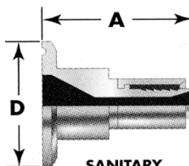
SANITARY JUMP SIZE STYLE 10U
